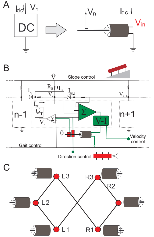
Fig. 6. CPG with integrated dynamics of the limb actuators into the gait control. A) Scheme showing the point of the circuit to get the values of functions V_n and I_{dc} in the case of DC block and motor. B) Feedback loop through the robot environment allowing to tune the central pattern generator according to the robot task. DC-block (Fig. 3) is substituted by the motor-leg-sensor block, voltage adder and voltage to current converter. New parts are shown in green. C) Ring configuration. Filled circles correspond to electrical circuits with the motor dynamics replacing the double capacitor in the circuit.
