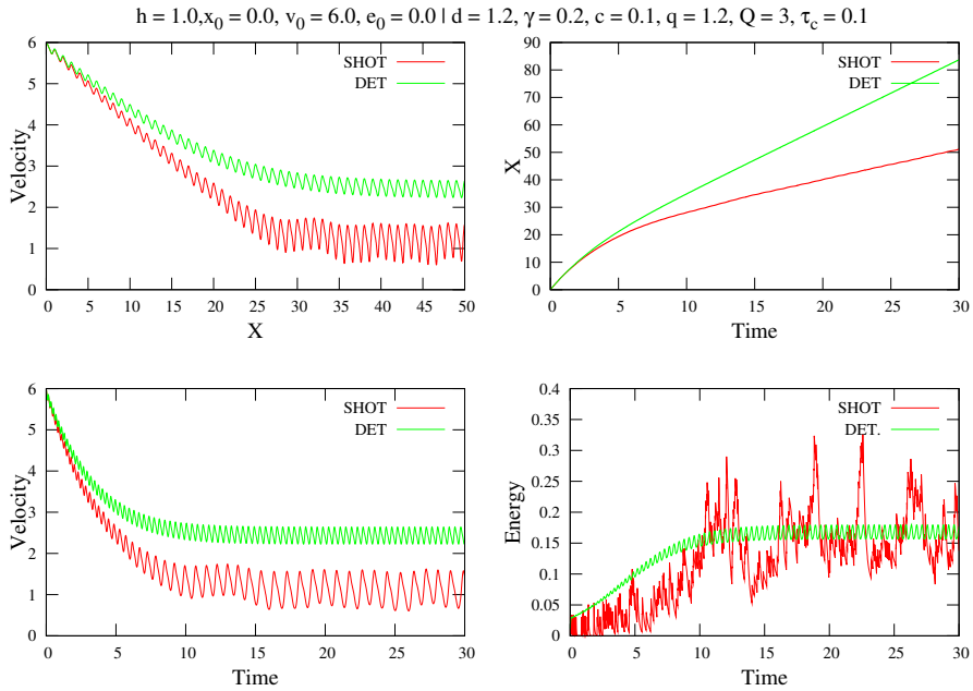
Fig. 9. Dynamics of particles on a flat Mateos' ratchet ( h = 1 ), which is driven by Poissonian noise with mean distance between shots \langle \delta t = 0.1 \rangle . The left panels show the velocity energy as a function of the coordinated and of the time, respectively. The right panels show: above - the coordinate as a function of time and below - the energy content of the reservoir as a function of time. Each of the figures shows a comparison of the shotnoise-driven ratchet with a ratchet driven by a continuous input q = 1.2 .
