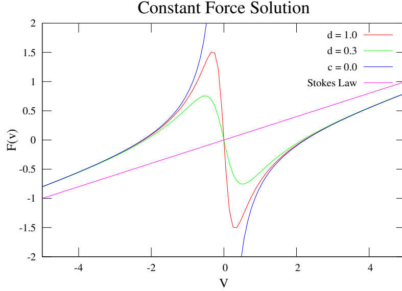
Fig. 2. Stationary solution: The force F_0 = -a as a function of the velocity for \gamma = 0.2 and 2 fixed d -values ( d = 0.3 and d = 1 with c = 0.1 ) and the asymptotic curve with c = 0 . The comparison is made with Stokes law F = \gamma v . The solution representing free motion corresponds to the roots on the axis F = 0
