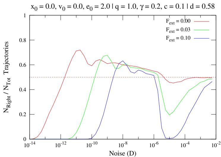
Fig. 8. Example of noise influence on the fraction of particles moving right in average over a time T \simeq 300 in dependence on the noise strength for different tilts.
