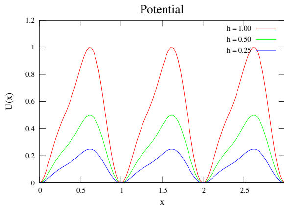
Fig. 1. Ratchet potentials of the type proposed by Mateos et al. [24, 25] with different height h = 1.0, 0.5, 0.25
