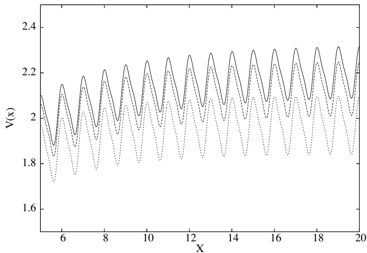
Fig. 6. Example of an unidirectional flux in a Mateos ratchet with h = 0.2 and the driving parameters q = 1, c = 0.1, d = 1 for a series of tilts with increasing loads a = 0, 0.03, 0.1 . With increasing load the velocity decreases, however downhill motion is impossible.
