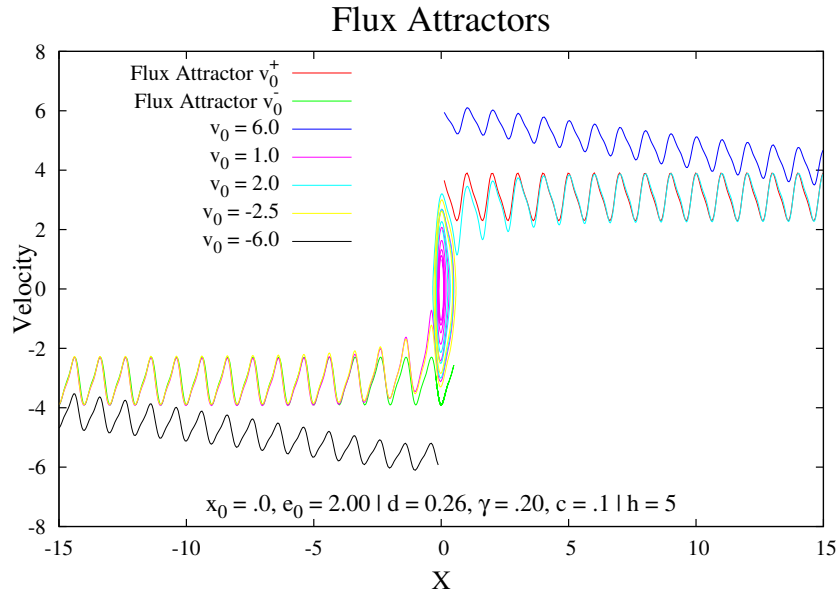
Fig. 3. Examples for trajectories which go to different attractors starting from different initial velocities. Due to the ratchet asymmetry negative initial velocities can give rise to positive asymptotic ones and vice versa.
