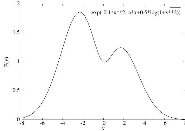
Fig. 7. Example of an unsymmetrical velocity distribution corresponding to a flux on the tilted ratchet. The downhill motion has a higher probability.
