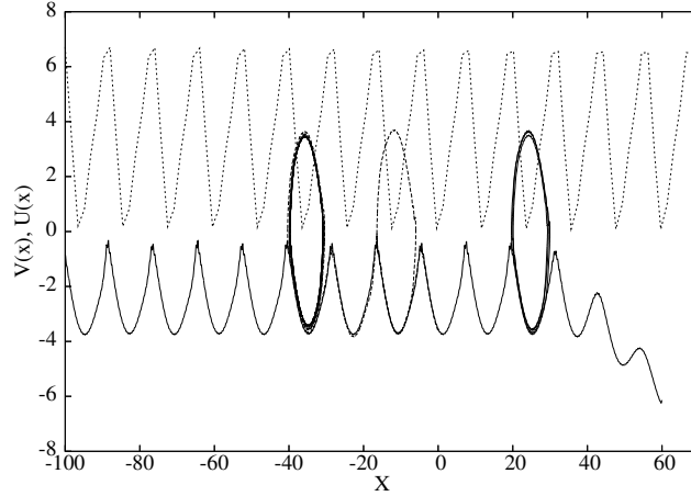
Fig. 4. Simulation results for a very steep Mateos ratchet h = 7 which is shown above. The parameters of driving are q = 1, c = 0.1, d = 1.2 . Two trajectories are shown, the first one makes a transient limit cycle and then is running to the left. A second trajectory starting from a different initial condition is trapped first in a transient cycle and then in a stable limit cycle.
